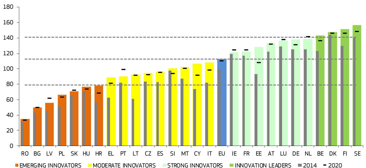
Figure 1: Global performance
