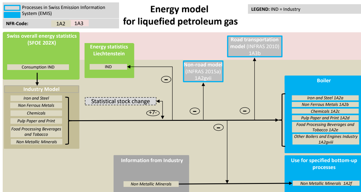
Figure 3-15 Schematic disaggregation of fuel consumption for liquefied petroleum gas.
