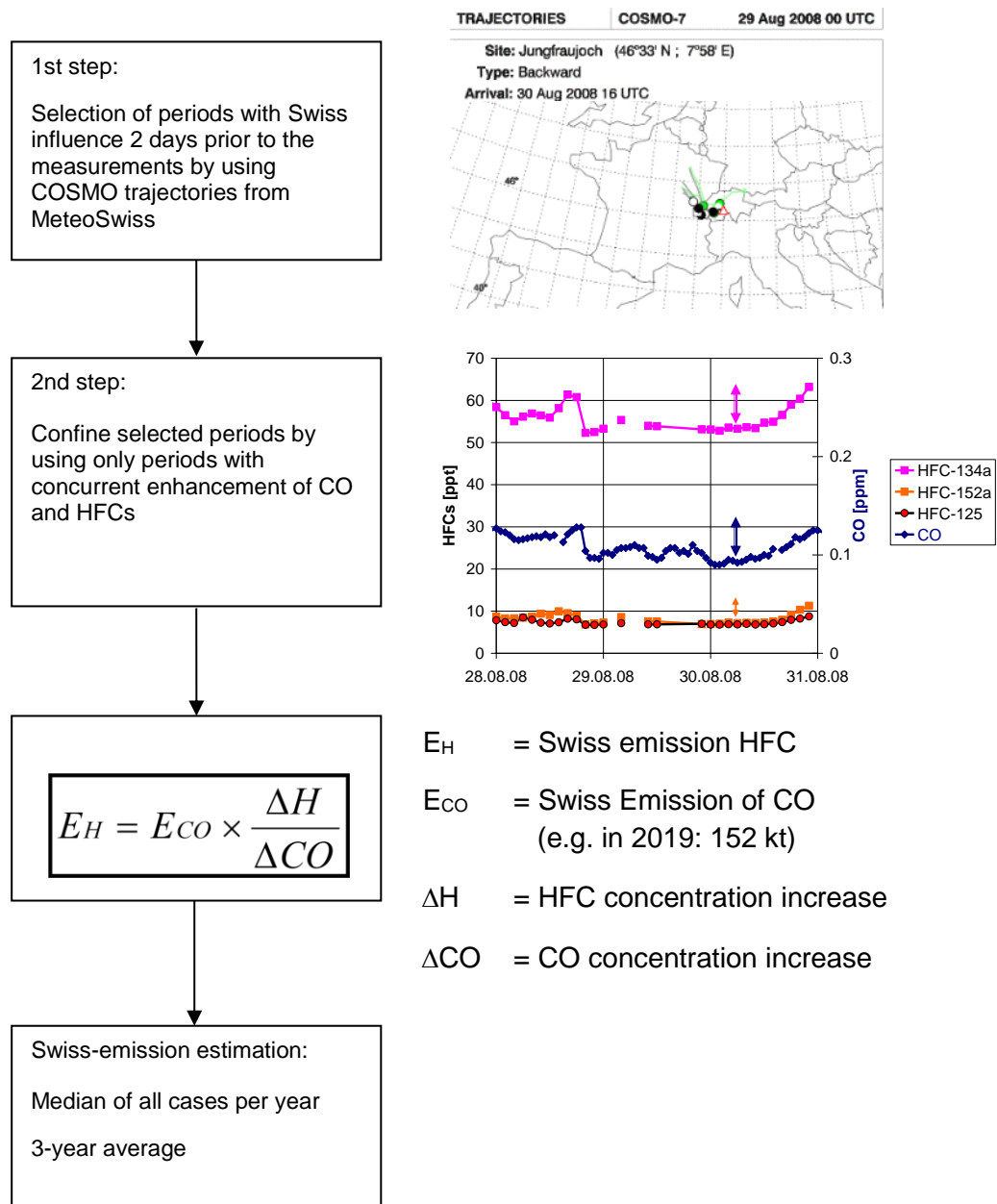
Figure A – 3 Description of the procedure to estimate annual emissions of halogenated greenhouse gases from Switzerland by using continuous measurements of HFCs at Jungfrauoch (Switzerland). Swiss emission of CO ( E_{CO} ) values are taken from FOEN (2021b), see chp. 3.2.4.1 concerning system boundaries.
