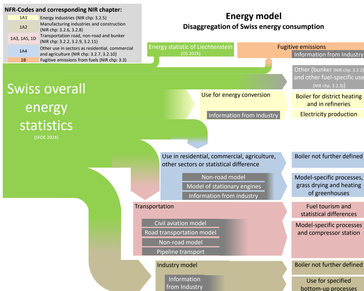
Figure 3-9 Overview of Switzerland's energy model. In the abbreviations SFOE 202X and OS 202X the "X" refers to the latest edition of the respective statistics.
