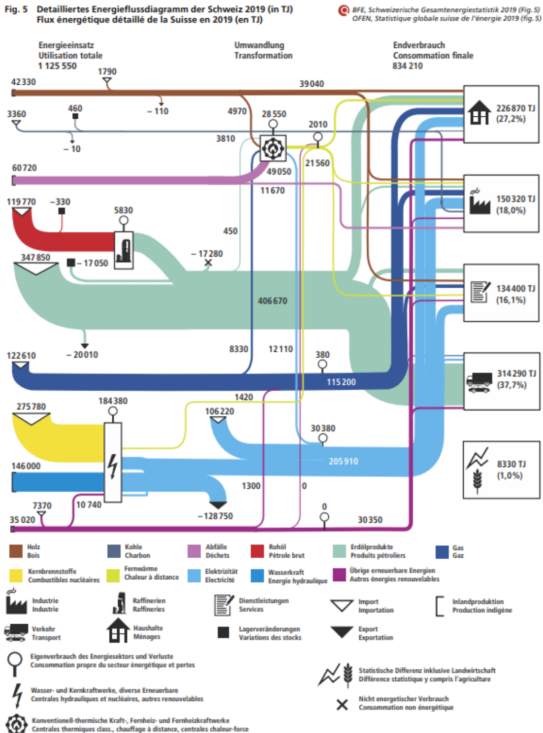
Figure A – 2 Energy flow in Switzerland 2019 in TJ (SFOE 2020)
