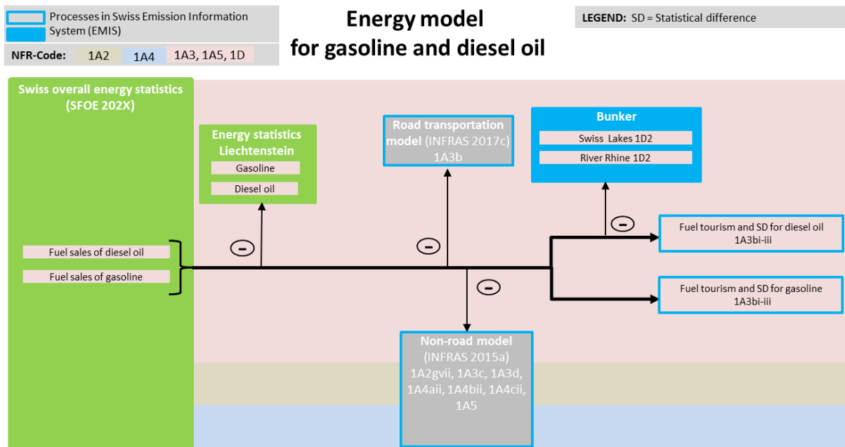
Figure 3-11 Schematic disaggregation of fuel consumption for gasoline and diesel oil. Marine bunker fuel consumption is based on the national customs statistics (see chp. 3.2.2.2.2). In the greenhouse gas inventory, emissions from 1A3bviii Fuel tourism and statistical differences are reported in the source categories 1A3bi, 1A3bii, and 1A3biii (see chp. 3.2.9.2.2 for a more detailed description).
