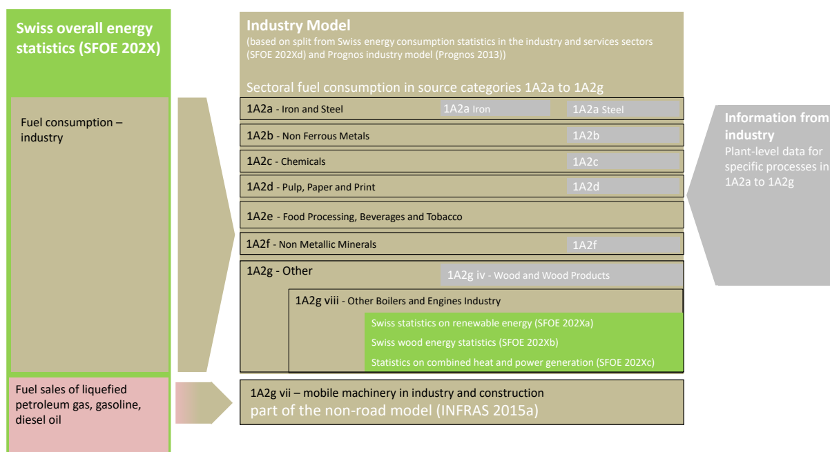
Figure 3-23 Schematic presentation of the data sources used for the industrial sectors 1A2a–1A2g. The references SFOE 202X, 202Xa, 202Xb and 202Xc refer to the 2020 edition of the corresponding energy statistics. For each fuel type, the Swiss overall energy statistics provide the total consumption for industry. The total consumption is then distributed to the different source categories based on information from industry surveys (SFOE 2020d) and the Prognos industry model (Prognos 2013). The grey boxes on the right show the specific bottom-up industry information.
