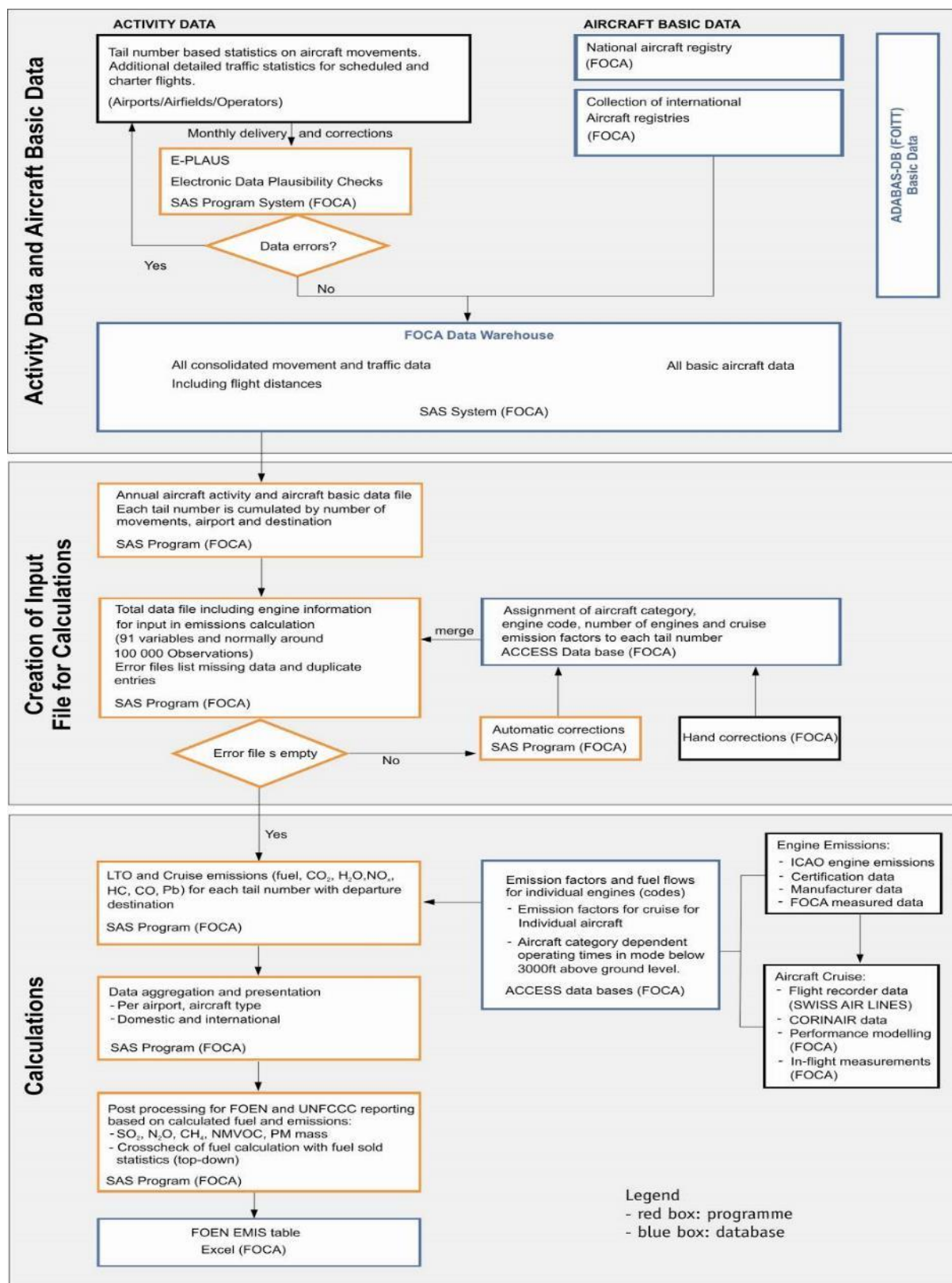
Figure 3-25 Modelling scheme (activity data, emission factors, emissions) for domestic aviation.
