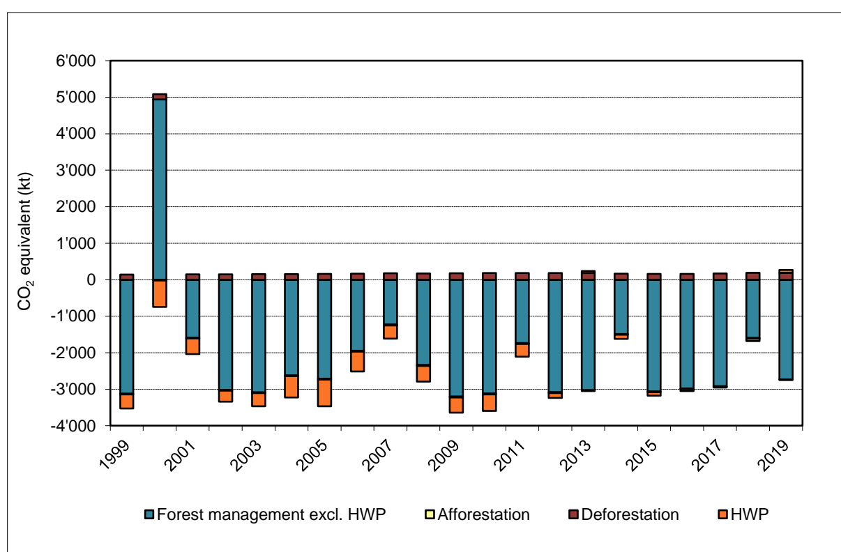
Figure E- 3 Greenhouse gas emissions (positive sign) and removals (negative sign) from Afforestation (too small to be distinguishable) and Deforestation under Article 3, paragraph 3, Forest management excluding HWP, and HWP under Article 3, paragraph 4.
