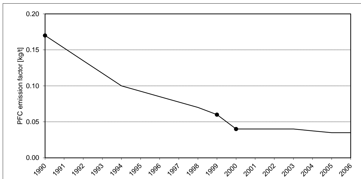
Figure 4-6 Extrapolation of PFC emission factor based on measurements in 1990, 1999 and 2000. The path for the reduction between measurements and the stagnation after the last measurements reflects the observed development of average EFs in the European Union.
