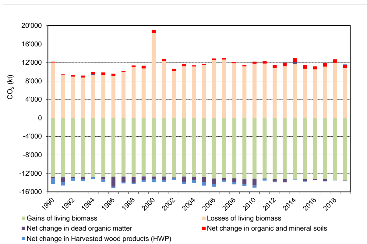
Figure 6-1 CO 2 emissions and removals in the LULUCF sector (in kt CO 2 ) broken down by (1) CO 2 removals due to carbon gains in living biomass, (2) CO 2 emissions due to carbon losses in living biomass, (3) net CO 2 changes in dead organic matter, (4) net CO 2 changes in organic and mineral soils, and (5) net CO 2 changes in Harvested wood products. Positive values refer to net emissions, negative values refer to net removals.
