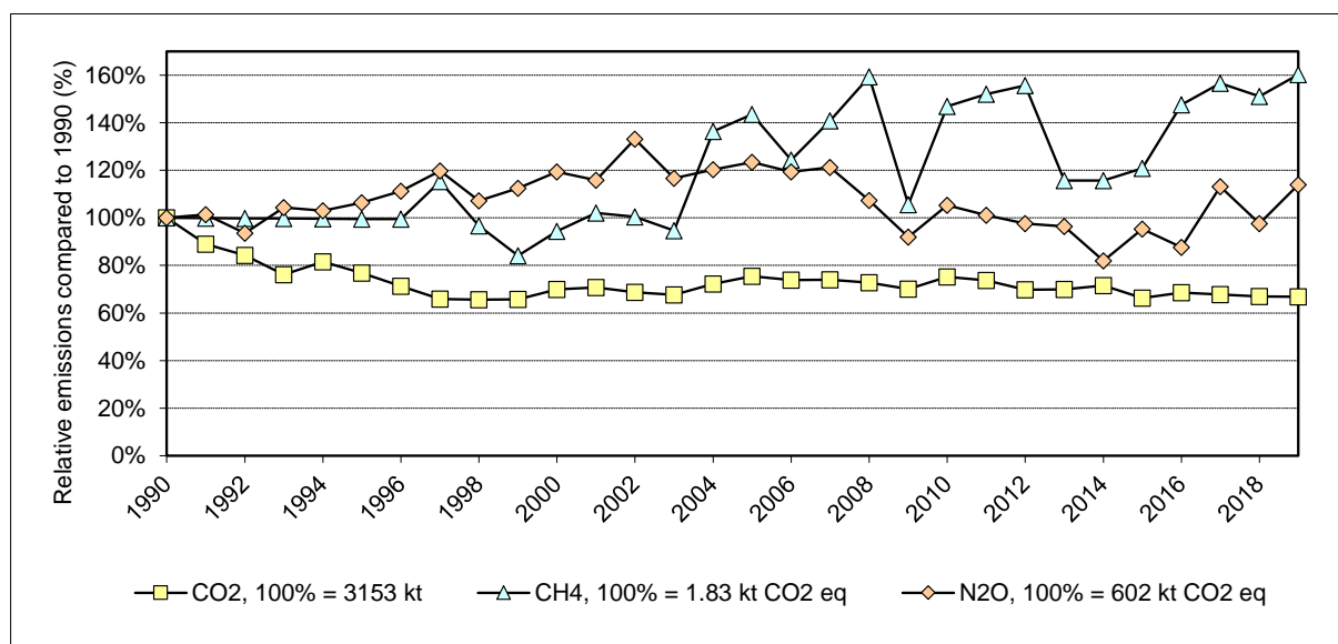
Figure 4-2 Relative trends of the greenhouse gas emissions (without F-gases, see Figure 4-3) of sector 2 Industrial processes and product use. The base year 1990 represents 100%.
