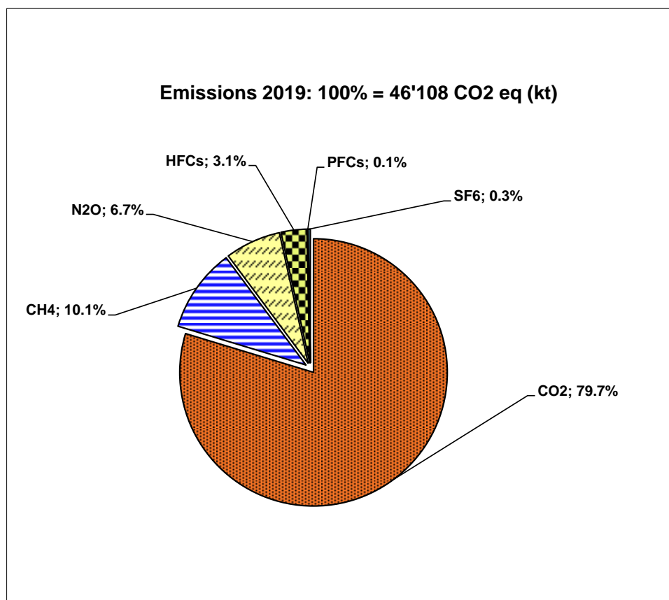
Figure 2-1 Contribution of individual gases to total greenhouse gas emissions in 2019 (excluding LULUCF, excluding indirect CO 2 ).
