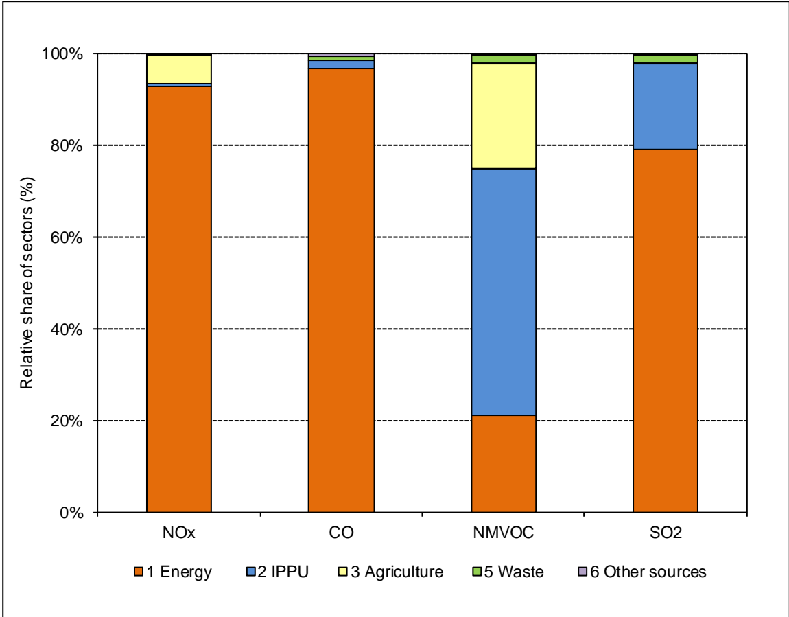
Figure 2-11: Relative contributions of individual sectors to precursor gas emissions in 2019 (excluding LULUCF).
