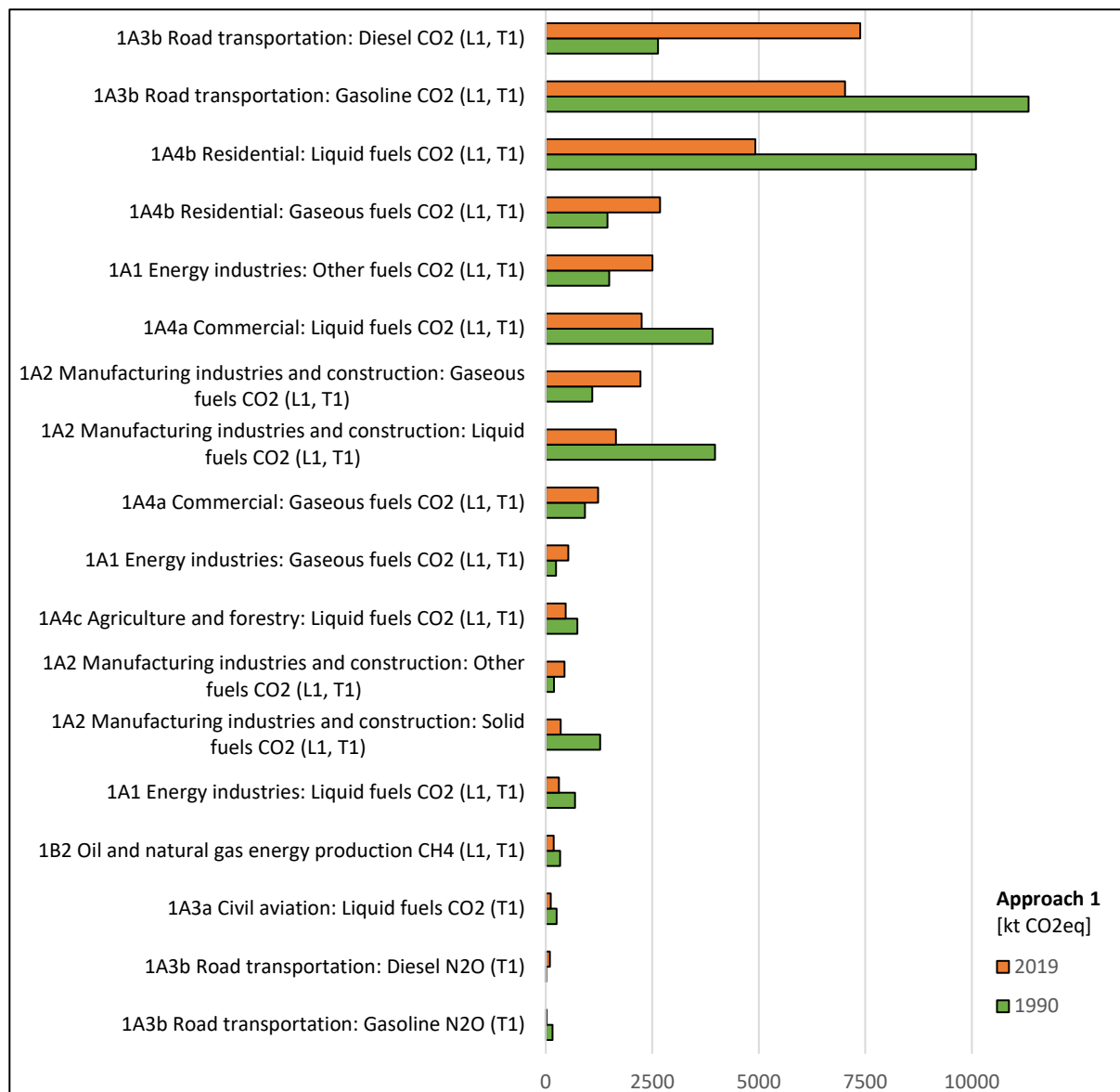
Figure 3-3 Key categories in the Swiss GHG inventory from sector 1 Energy determined by Approach 1 (L1 = key category according to Approach 1 level in 2019; T1 = key category according to Approach 1 trend 1990–2019).
