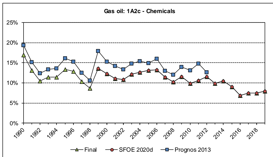
Figure 3-24 Illustrative example for combining time series with consistent overlap according to the 2006 IPCC Guidelines (IPCC 2006, Volume 1, chp. 5). The y-axis indicates the share of source category 1A2c of total gas oil consumption in the industry sector. The green triangles correspond to the share finally used to calculate the fuel consumption in 1A2c, based on the combination of the shares from the energy consumption statistics in the industry and services sectors (SFOE 2020d, orange dots since 1999) and the bottom-up industry model (Prognos 2013, blue squares from 1990 to 2012). Similar calculations are performed for each source category and fuel type.
