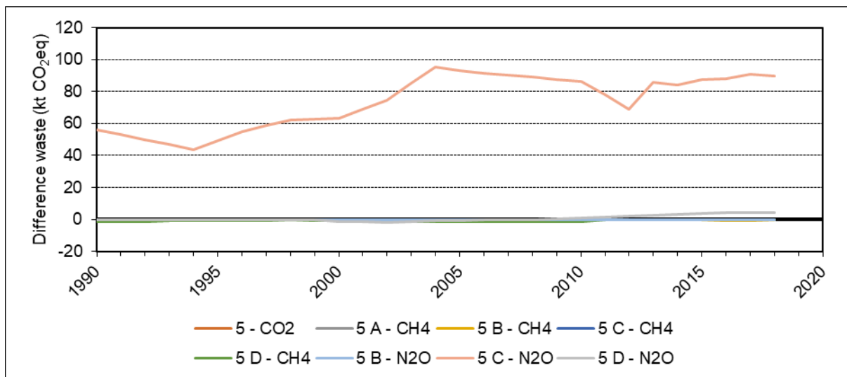
Figure 10-17 Differences in CO 2 , CH 4 , N 2 O emissions (in kt CO 2 eq) between the latest and the previous submissions for sector Waste. Positive values refer to higher emissions and negative values to lower emissions in the latest submission compared to the previous submission.
