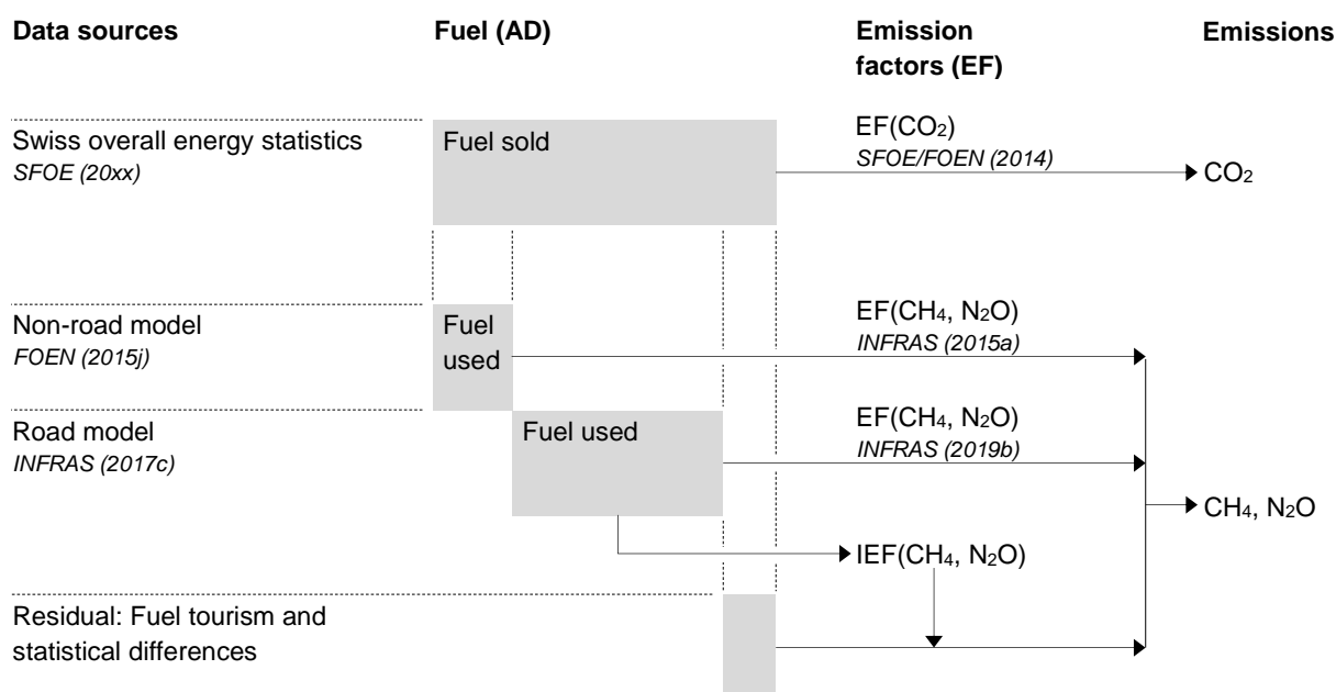
Figure 3-26 Connections between fuel sold and fuel used for road and non-road transportation. Fuel sold is provided by the Swiss overall energy statistics (minus Liechtenstein's gasoline and diesel oil consumption and bunker fuels for navigation). Fuel used results from the territorial road and non-road models. The residual fuel consists of fuel tourism and statistical differences. Its emissions are calculated by means of implied emission factors deduced from the territorial road model. The diagram holds separately for gasoline and diesel oil. SFOE (20xx) stands for the latest Swiss overall energy statistics.
