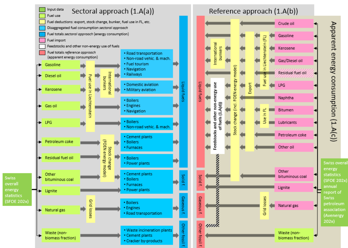
Figure 3-5 Calculation of Reference and Sectoral Approach. The input data for both approaches stem from the Swiss overall energy statistics (SFOE 2020). For the Reference Approach, additional information from Avenergy Suisse (formerly Swiss Petroleum Association) (Avenergy 2020) is used. While the Reference Approach considers the net import/export balance, the Sectoral Approach considers the fuel consumption. The dark grey arrows represent fuel deductions where occurring. The dashed arrow from the Feedstock use to Other fossil fuels stands for the CO 2 emissions from cracker by-products (originating from feedstock use of liquefied petroleum gas and naphtha) which are accounted for under Other fossil fuels. The graphic box of the import of Residual fuel oil is dashed since there is no more import of residual fuel oil.
